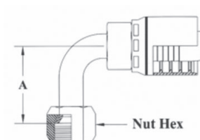
JIC 37° - 90° Female Swivel
