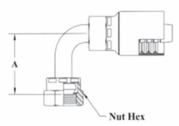
BSPP British Standard Parallel 60° Cone 90° Bend Female Swivel
