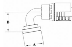
Code 61 Split Flange 100° Bend
