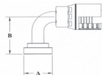
Code 62 Split Flange 90° Bend
