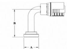
Code 61 Split Flange 90° Bend Long Drop
