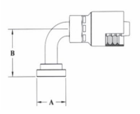
Code 61 Split Flange 90° Bend
