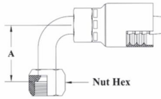
JIC/SAE Dual Seat 90° Female Swivel
