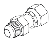
JIC to ORFS Swivel FF6504 Series Page N123
