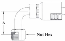
JIC/SAE Dual Seat 90° Female Swivel Long Drop
