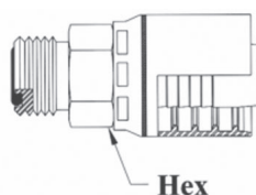
O-Ring Face Seal (ORF) Male Solid
