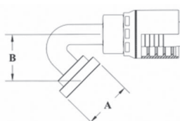
Code 61 Split Flange 135° Bend
