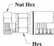
BSPP- British Standard Parallel 60° Cone - Female Swivel
