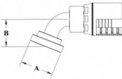
Code 61 Split Flange 67 1/2° Bend
