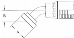
Code 62 Split Flange 45° Bend
