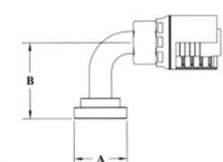
CODE 61 SPLIT FLANGE 90° BEND
