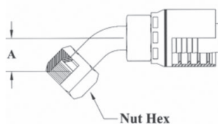
JIC 37° - 45° Female Swivel
