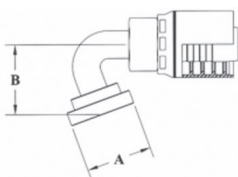
Code 61 Split Flange 110° Bend
