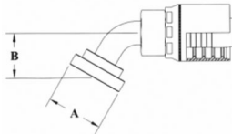
Code 61 Split Flange 67 1/2° Bend
