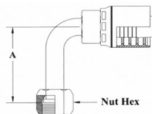
BSPP- British Standard Parallel 60° Cone - Female Swivel
