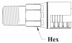
JIC 37° Male Solid
