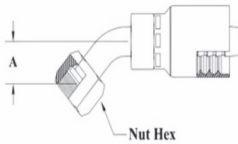
O-Ring Face Seal (ORF) 45° Female Swivel
