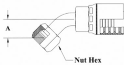
O-Ring Face Seal (ORF) 45° Female Swivel
