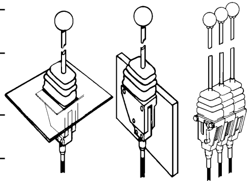
Flush Mounting Side Mounting Banked Together
